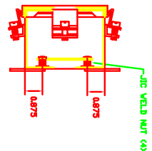
PANEL SIZE = A - 1.25, B - 1.125 DIC FIELD NUT (4)
